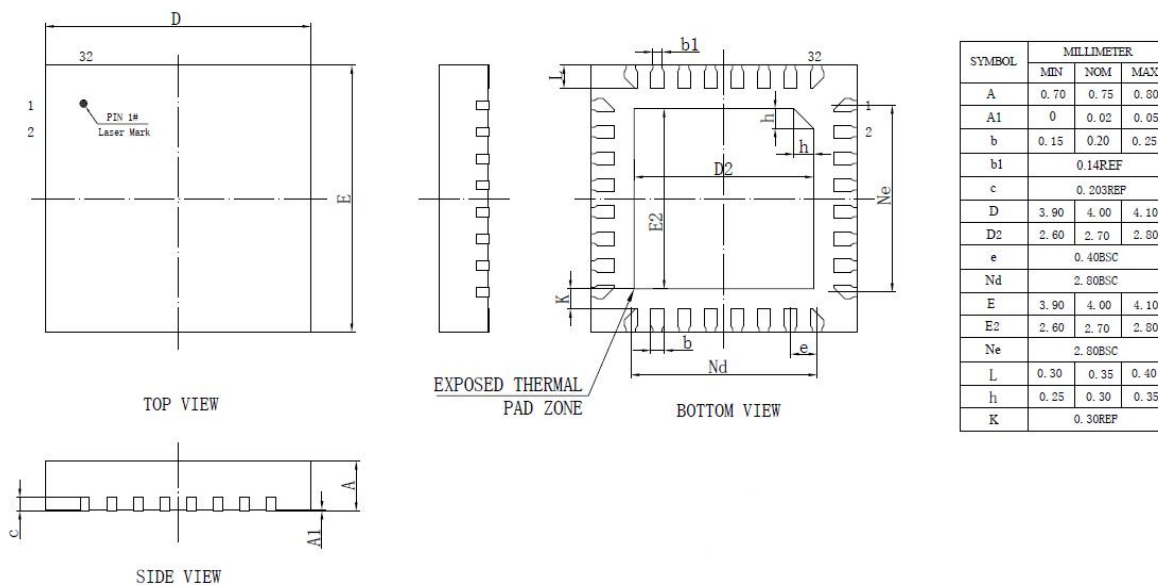
Figure 3-1 JL6976N8 Package
