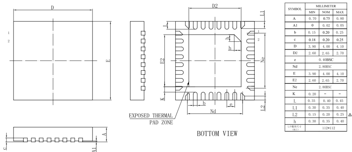
Figure 3-1 AC7006A Package
