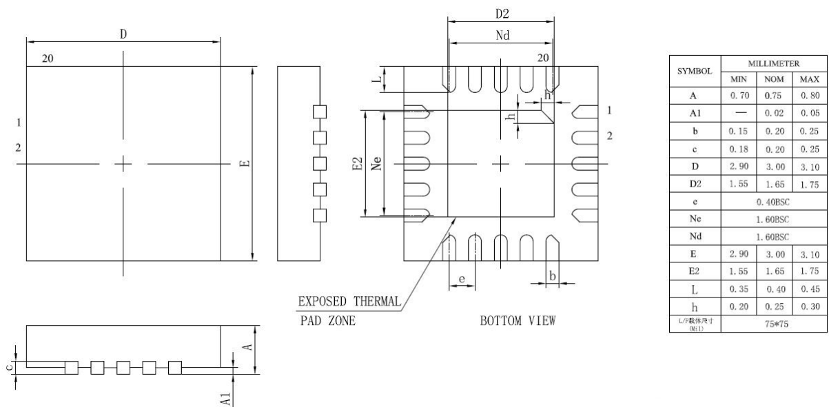
Figure 3-1 JL7003D Package
