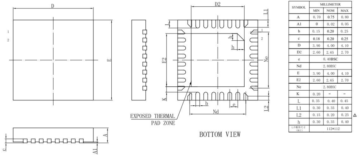
Figure 3-1 JL7016G Package
