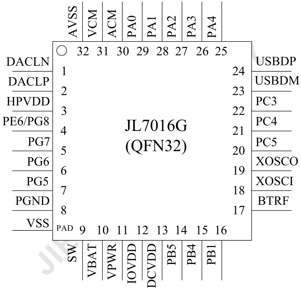
Figure 1-1 JL7016G Package Diagram
